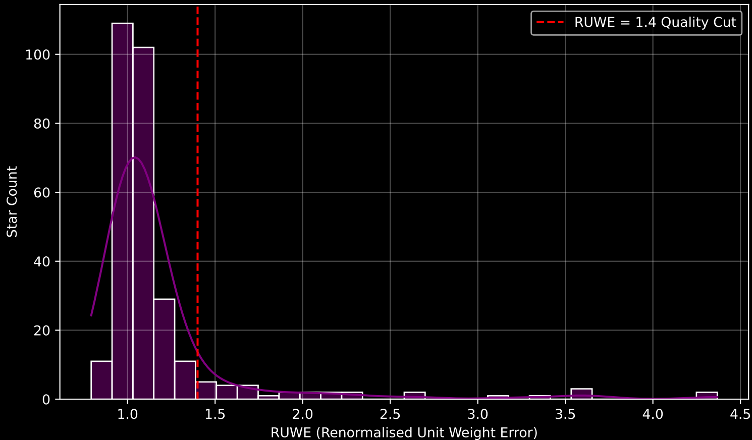
GAPOGEE DR17 Field [169-24_btx] RUWE Distribution (n= 293)
