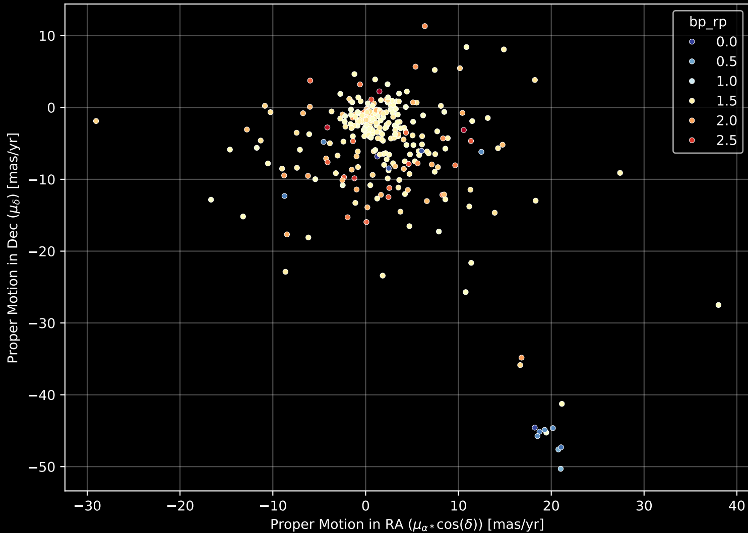
APOGEE DR17 Field: [169-24_btx] Proper Motion Diagram (n= 300)
