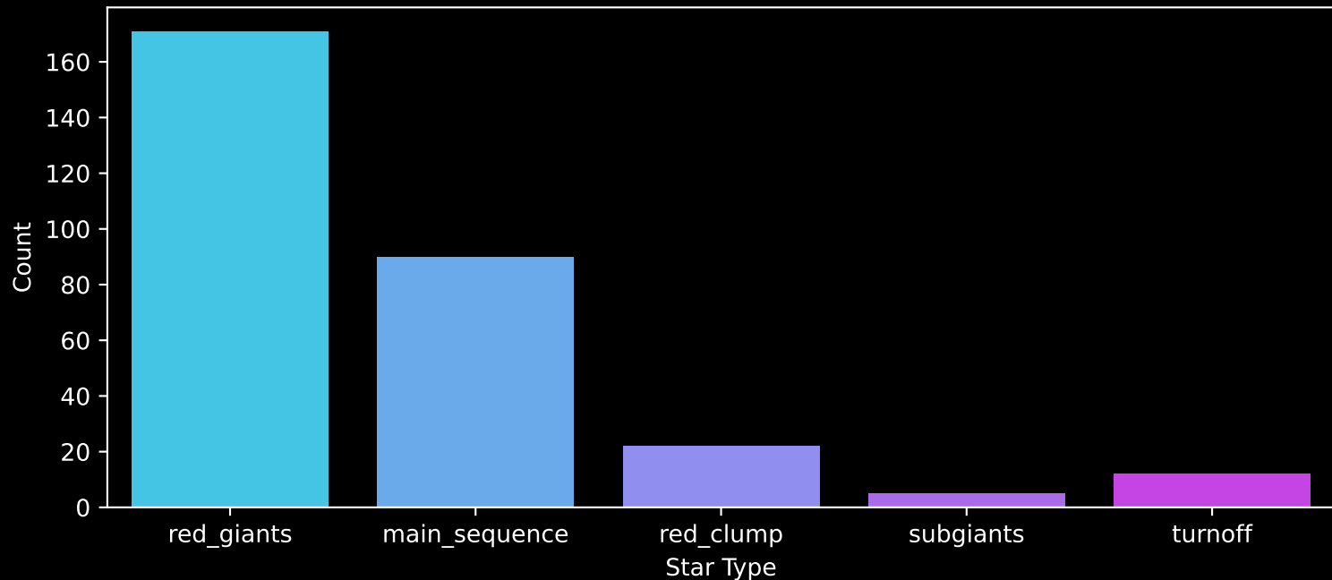
APOGEE DR17 Field: [169-24_btx] Count plot of Star Type
