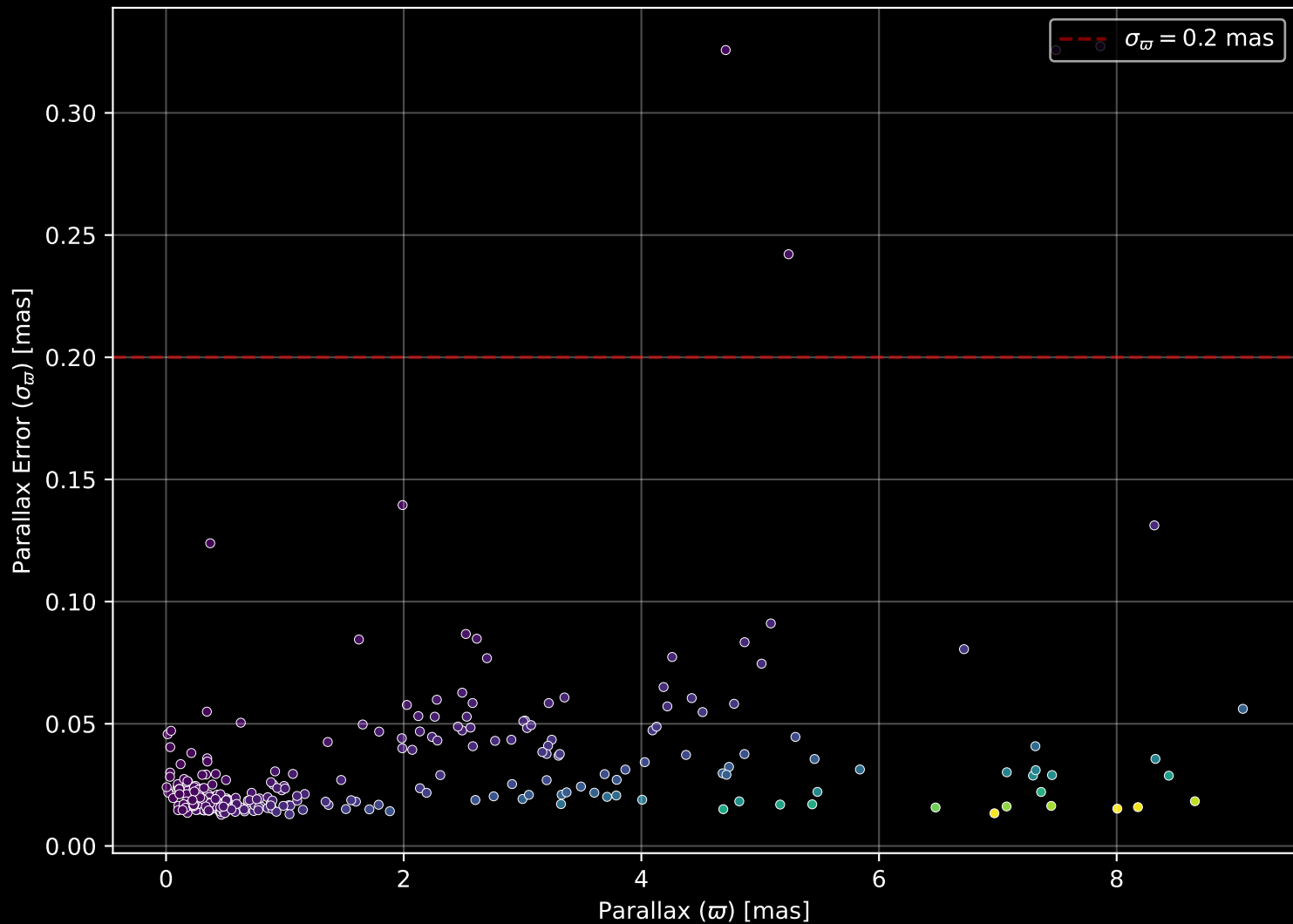
APOGEE DR17 Field: [169-24_btx] Parallax Quality (n= 300)
