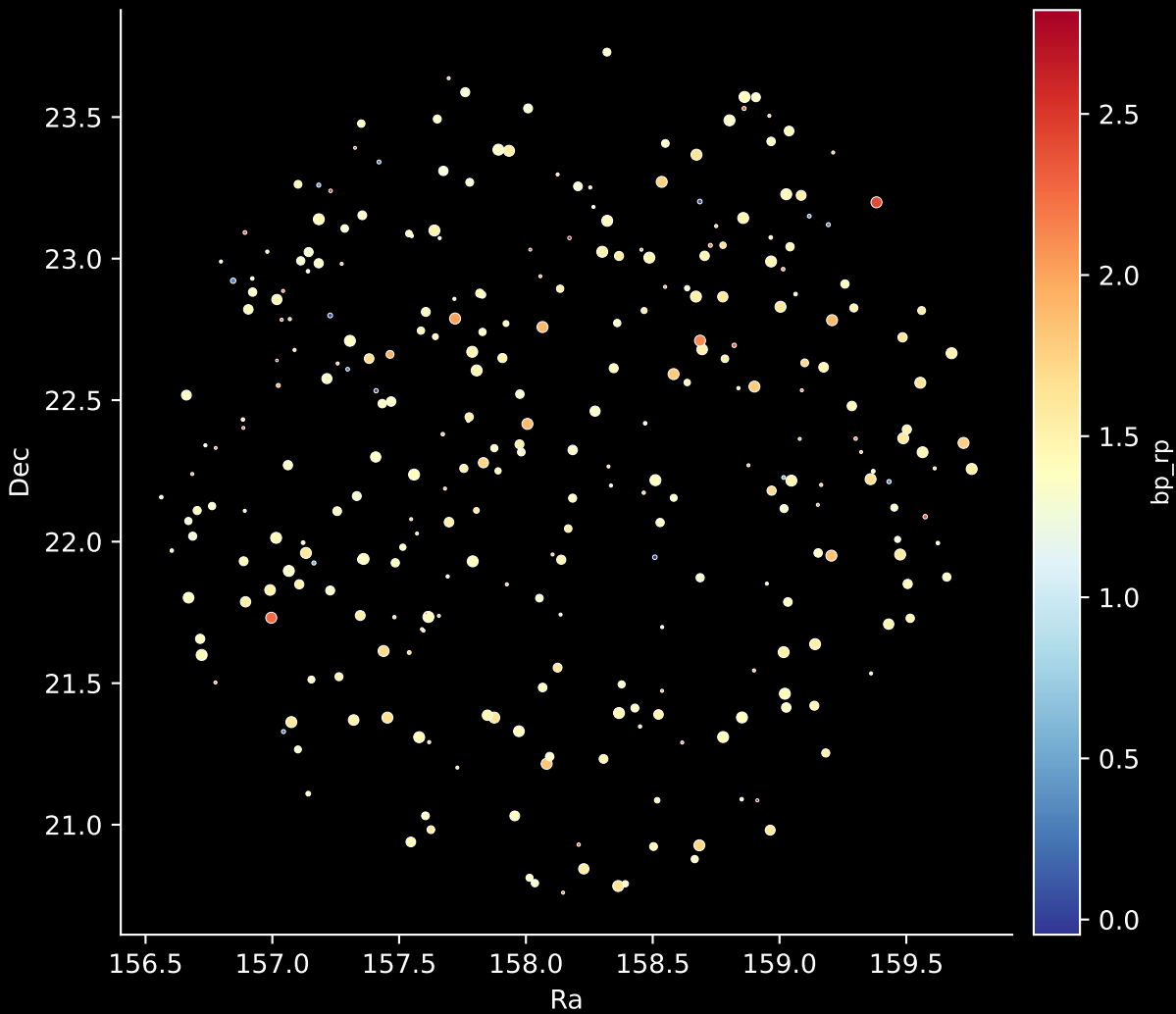
APOGEE DR17 Field: [169-24_btx] Stars: 300
