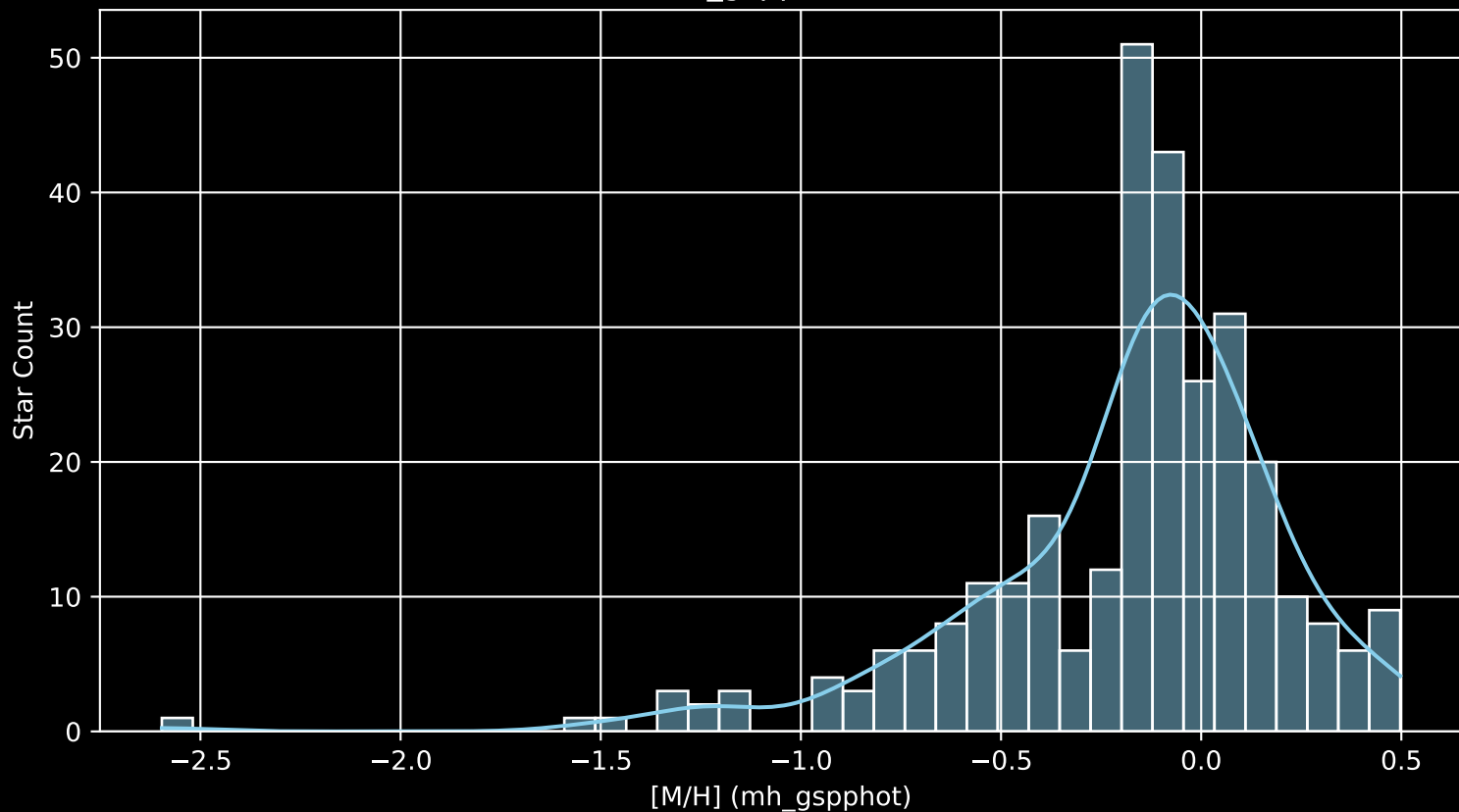
APOGEE DR17 Field: [169-24_btx [M/H] (mh_gspphot) (n= 298)
